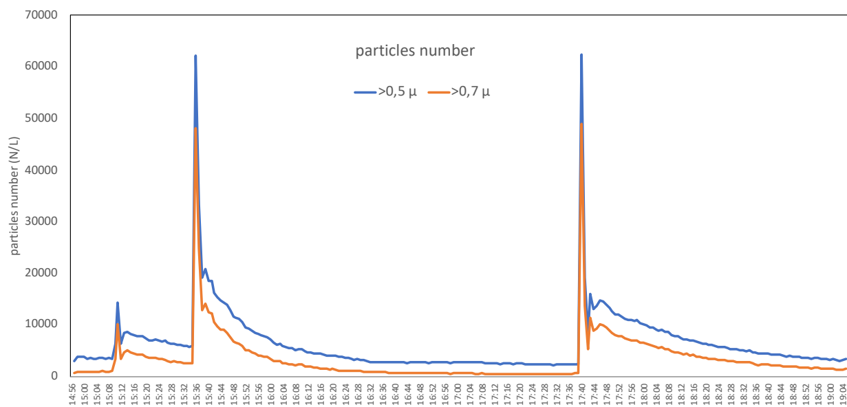
Fig. 7 – particles concentration trend (N/L)
