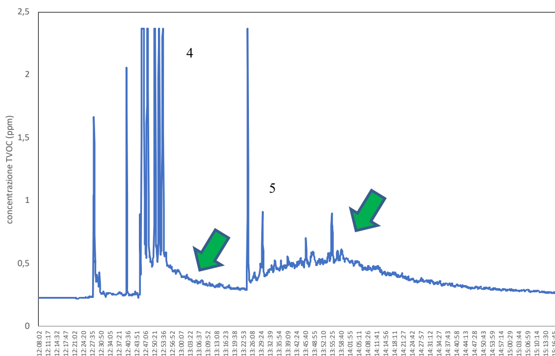
Fig. 3 – Trend of TVOC concentration (ppm): detail of fig. 2
