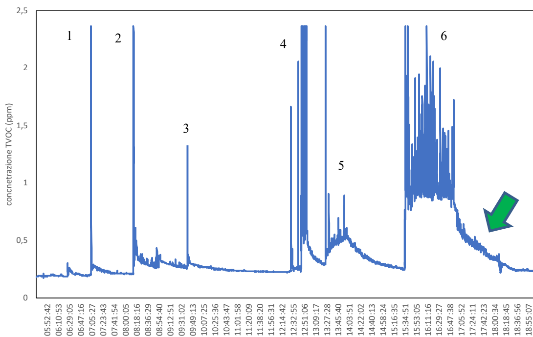
Fig. 2 – trend of TVOC concentration (ppm)
