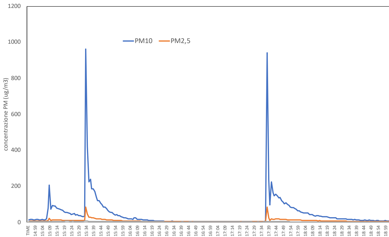
Fig. 4 –PM concentration trend
