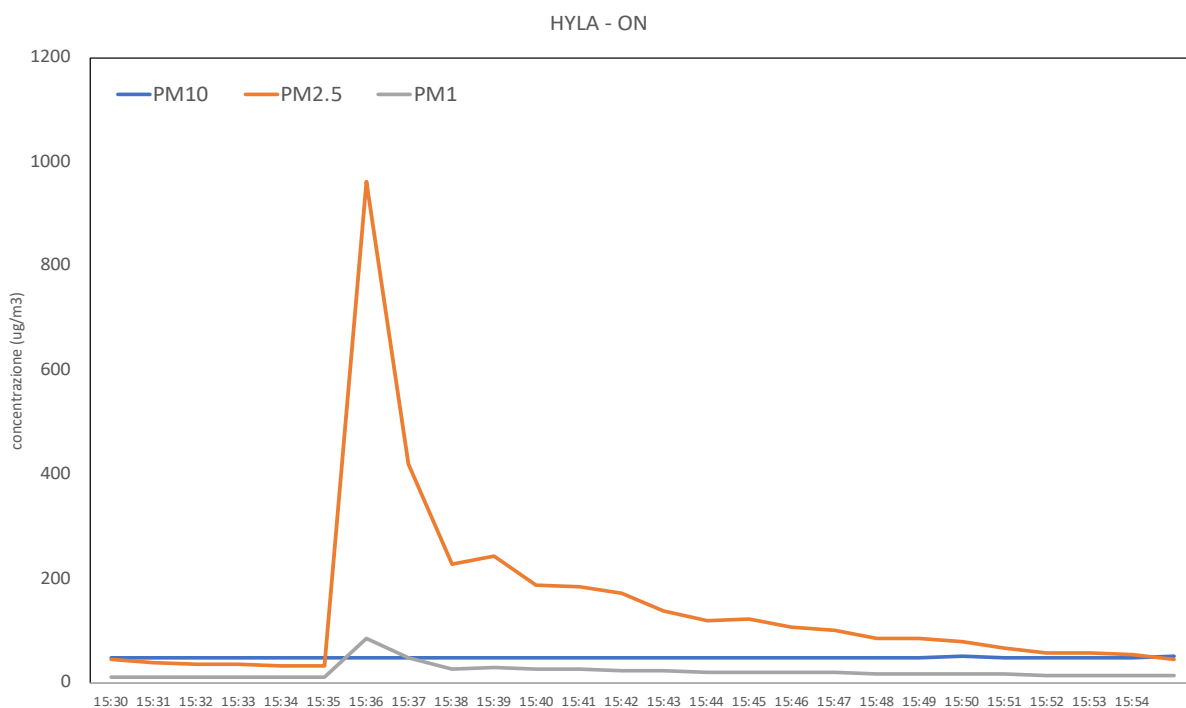
Fig. 5 – PM concentration trend with the HYLA device switched on
