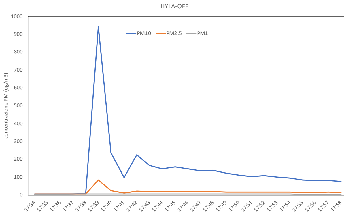
Fig. 6 – PM concentration trend with the HYL A device switched off
